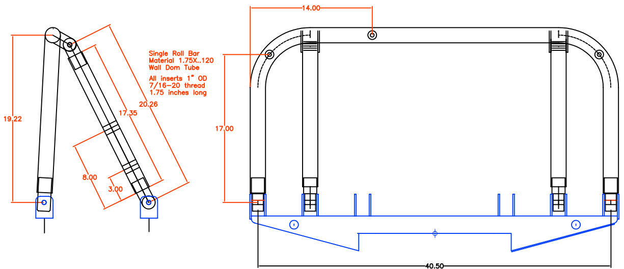
Full bar. 1.75 X .120 wall
